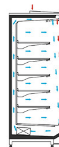
Air flow scheme for refrigerated cabinet Medusa Montenegro AC
