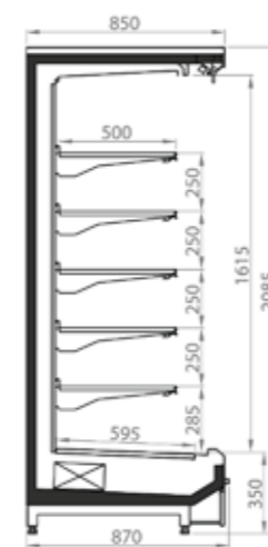
MEDUSA Montenegro Standard
