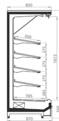
MEDUSA Montenegro Standard FV
