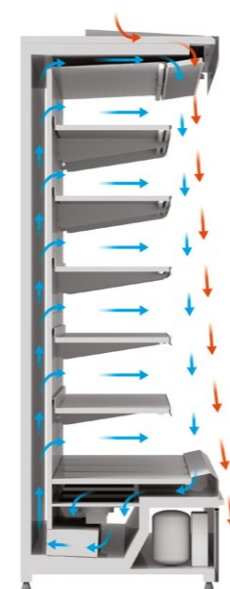
Air flow scheme for refrigerated cabinet Medusa Plug-in
