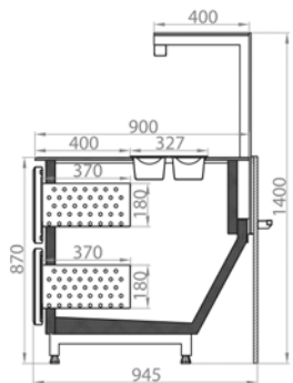
CUBE PIZZA Slim refrigeration cabinet
