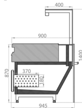
CUBE SO Slim (Fast-Food) refrigeration cabinet with integrated technological equipment
