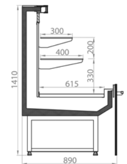
CASPIY CUBE Slim self-service refrigeration cabinet
