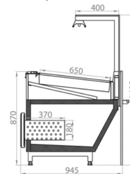
CUBE TC Slim hot cabinet for demonstration of ready meals
